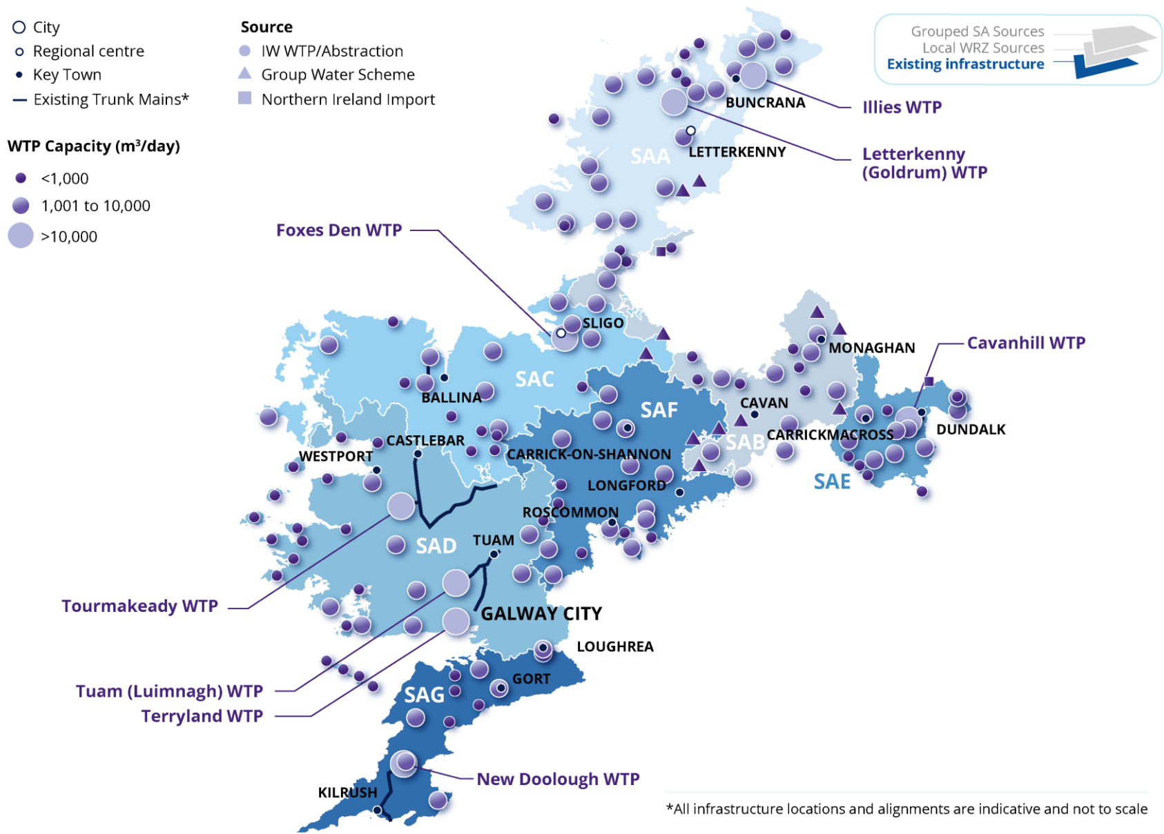
Figure 7.2 Existing Infrastructure
