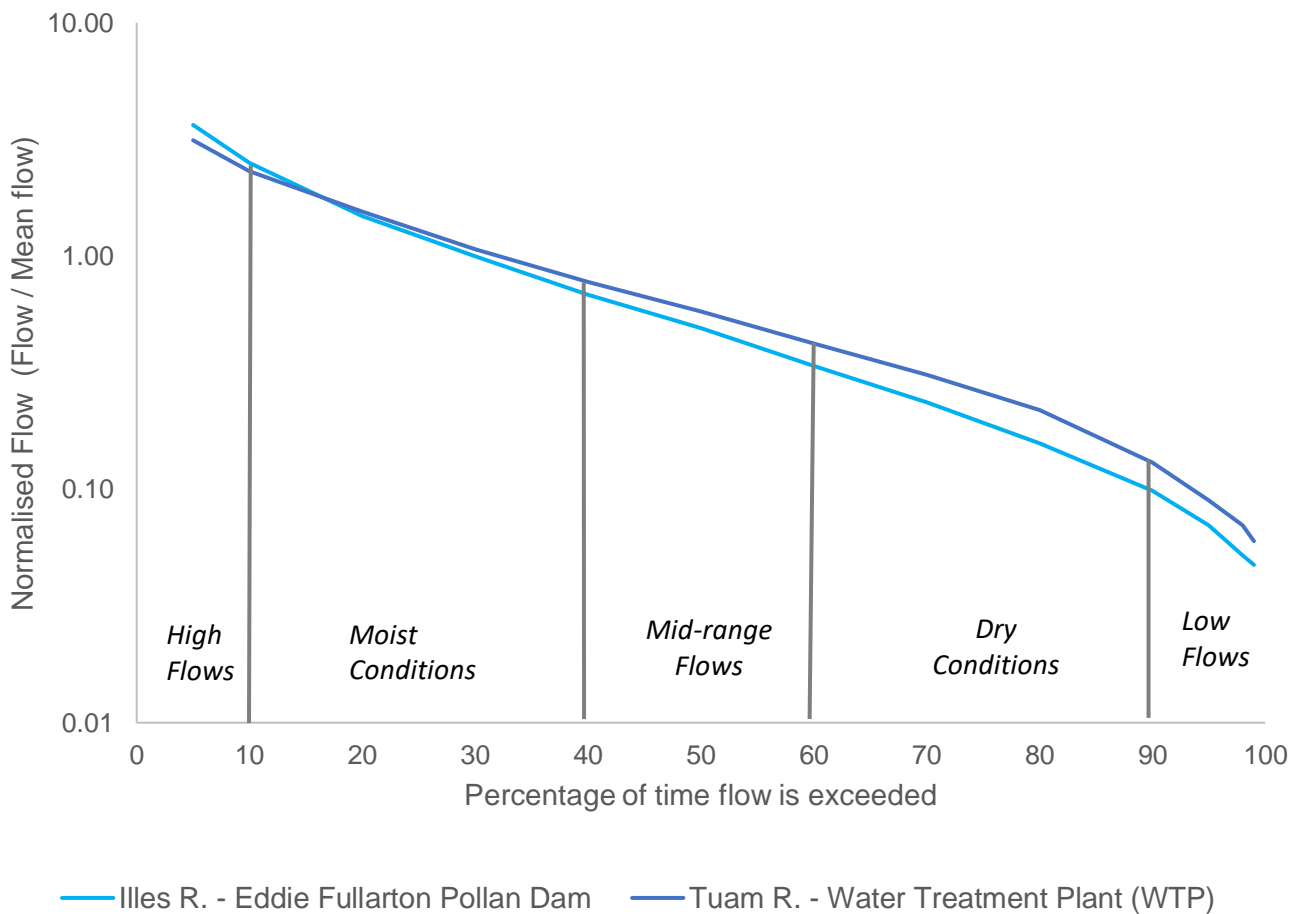
Figure 3.9 Hydrological Characteristics of the Illes River and Tuam River
