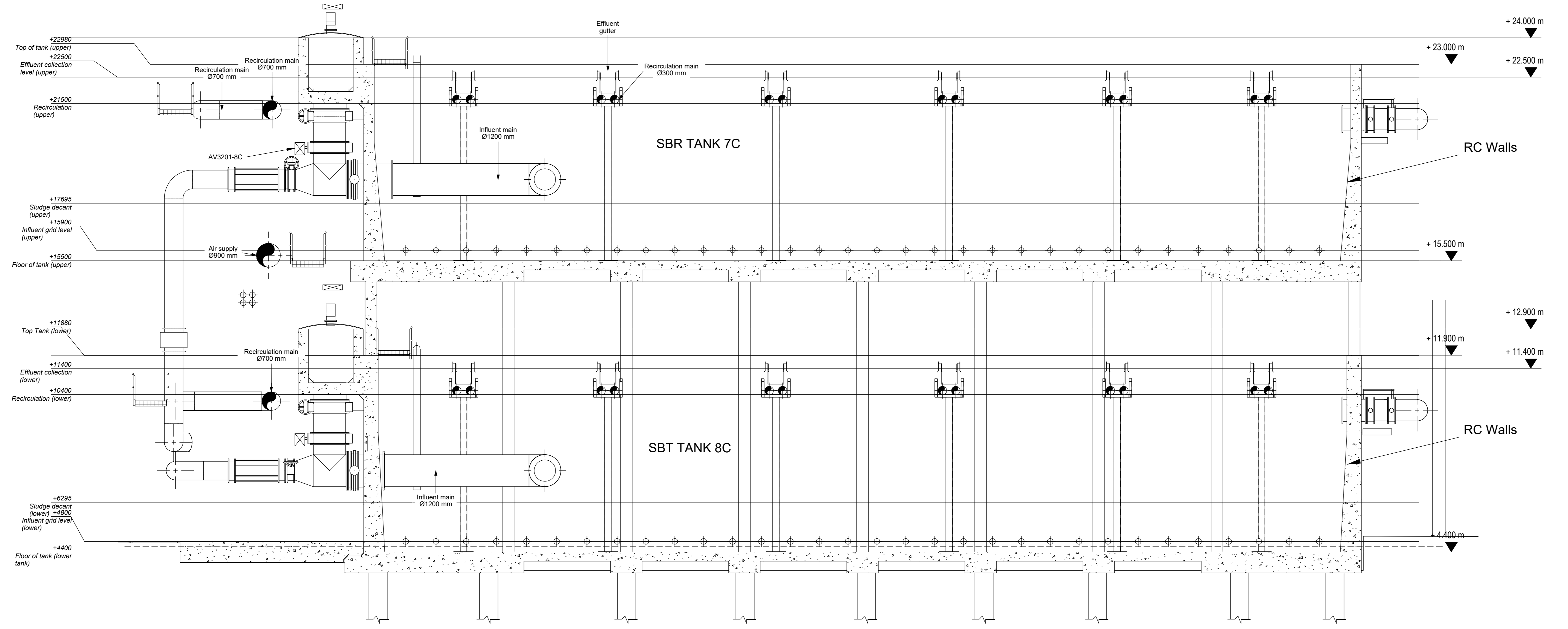
SECTION 1-1 Scale 1:75
