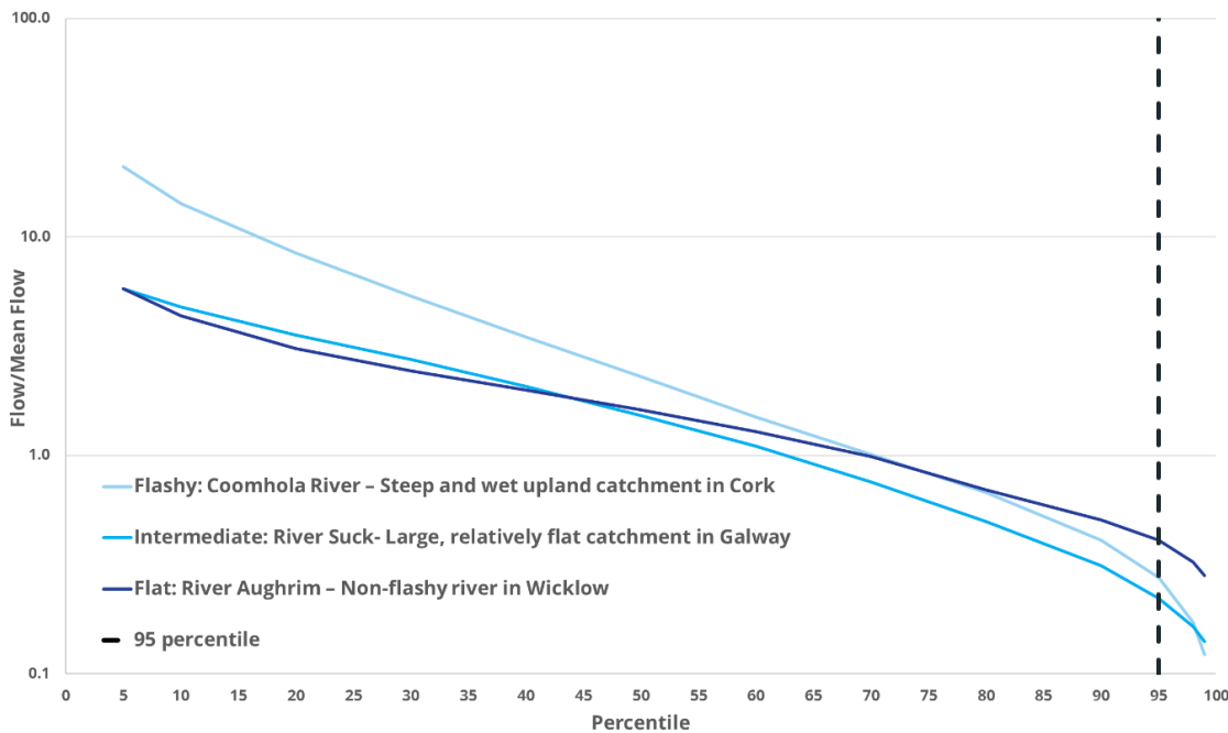
Figure 1-2 Example of a Flow Duration Curve
